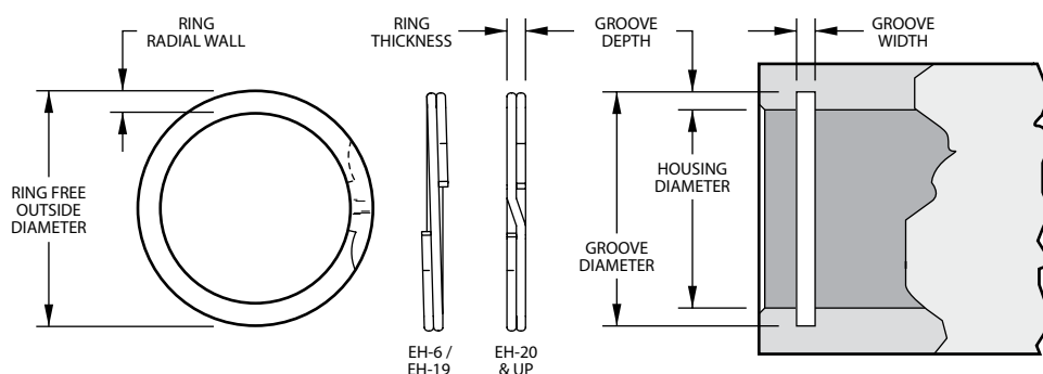
Product Dimensions All dimensions in millimeters unless otherwise specified.
